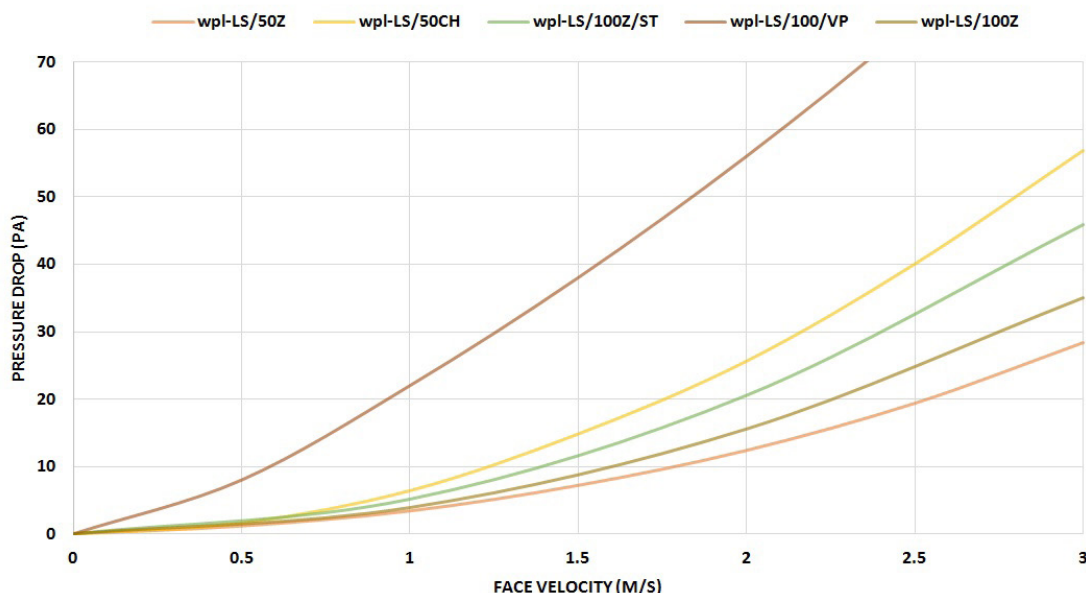
WPL (UK) - Louvre Blade Pressure Drops
